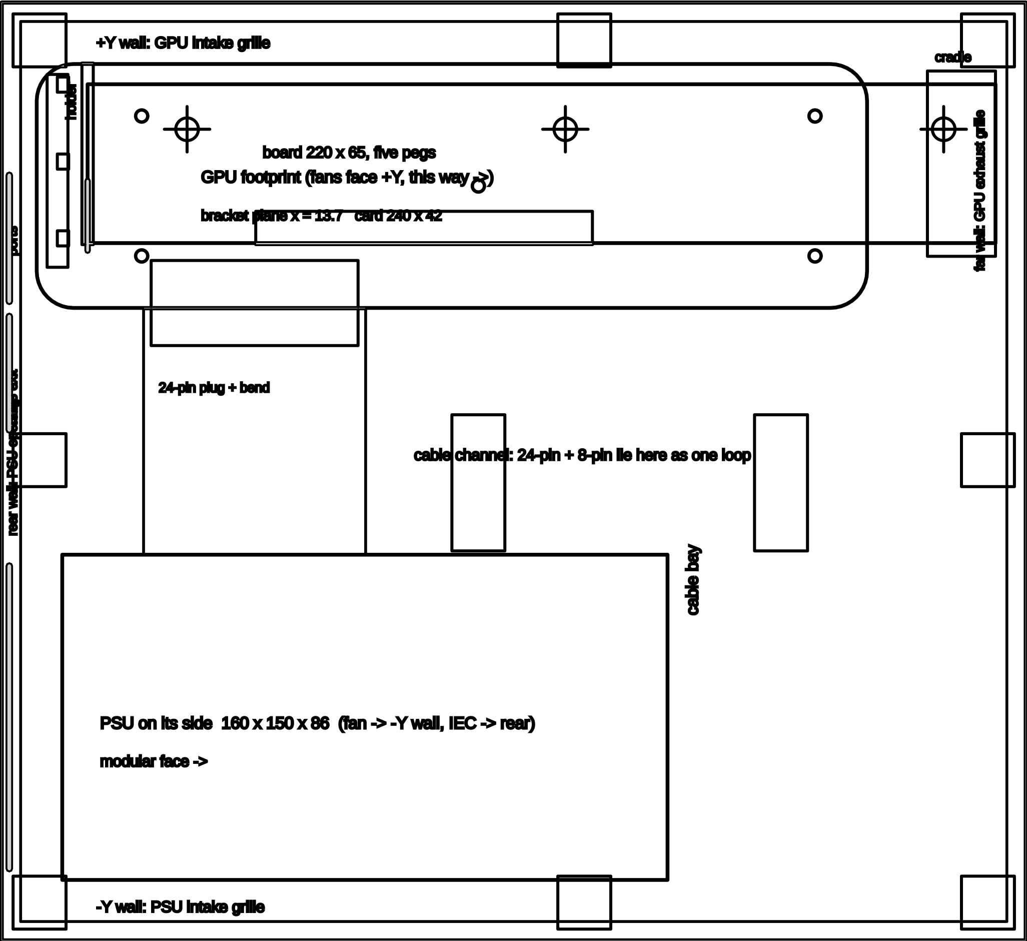
xgm-lite-frame floor plan 1:1 outside 270.7 x 248 mm (board origin = its rear/24-pin corner)
