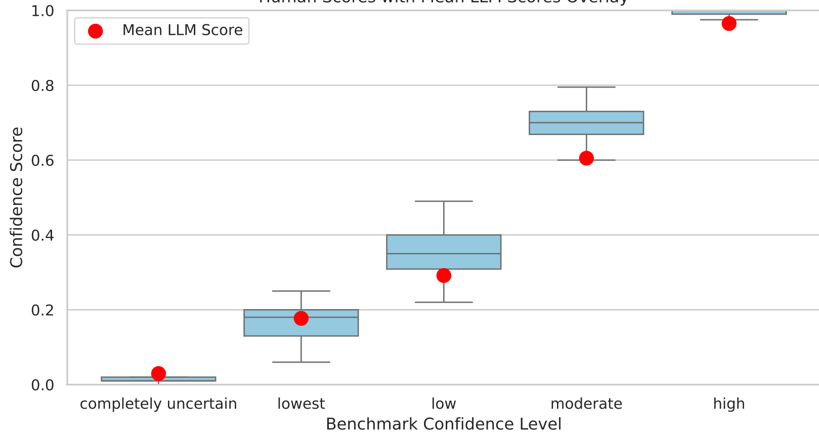
Human Scores with Mean LLM Scores Overlay
