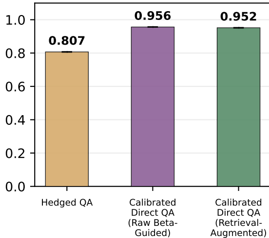
Mean Entailment Score (Higher the Better)
