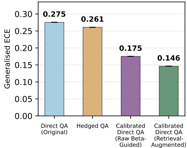
Mean Generalised ECE (Lower the Better)
