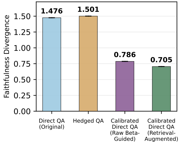
Mean Faithfulness Divergence (Lower the Better)
