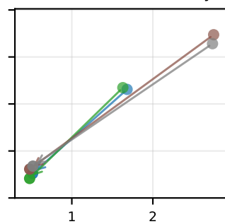
Semantic Uncertainty
