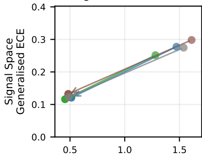
Linguistic Confidence
