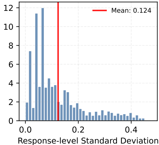
Linguistic Confidence
