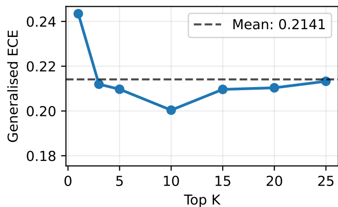
LC - Generalised ECE
