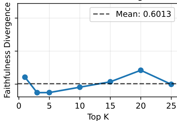
TP - Faithfulness Divergence
