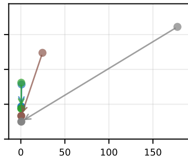
Token Probability
