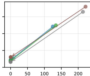
Semantic Uncertainty
