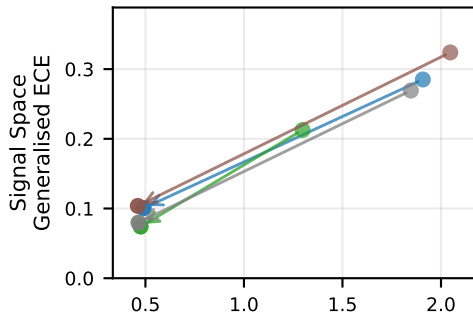
Linguistic Confidence
