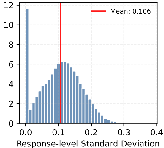
Token Probability
