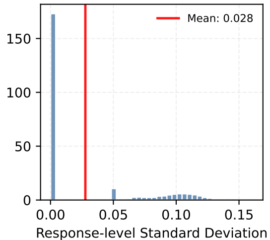
Semantic Uncertainty
