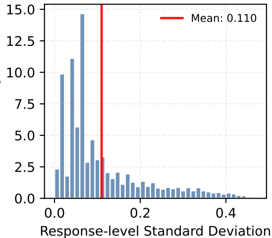
Linguistic Confidence
