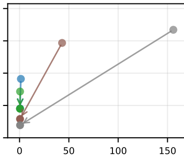
Token Probability
