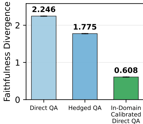
Mean Faithfulness Divergence (Lower the Better)
