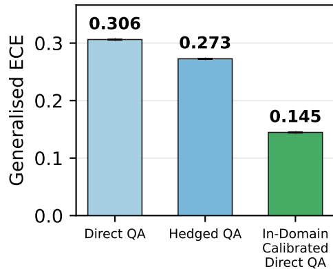
Mean Generalised ECE (Lower the Better)
