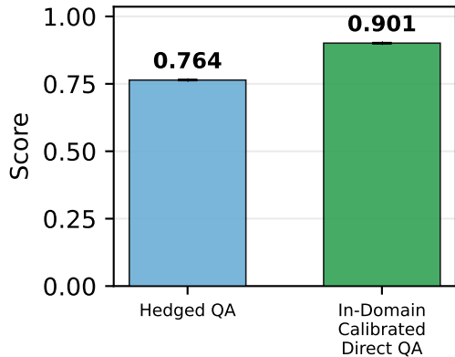
Mean Entailment Score (Higher the Better)
