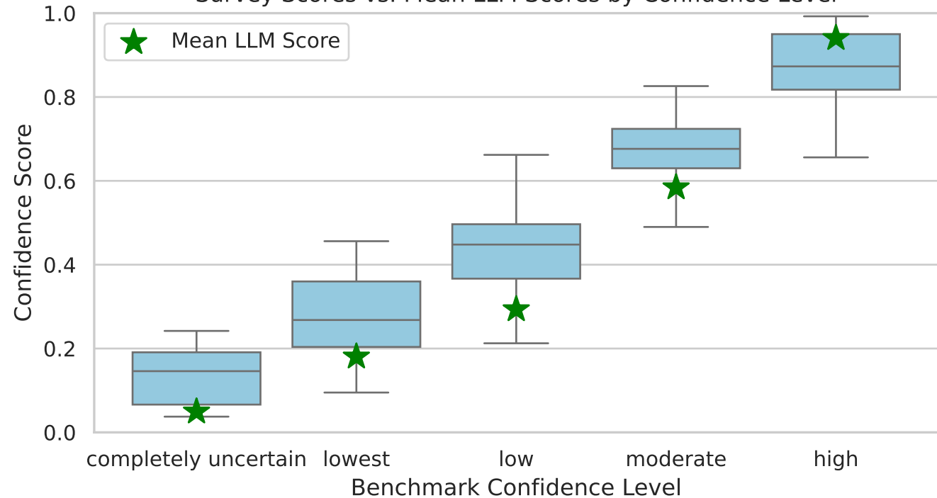
Survey Scores vs. Mean LLM Scores by Confidence Level
