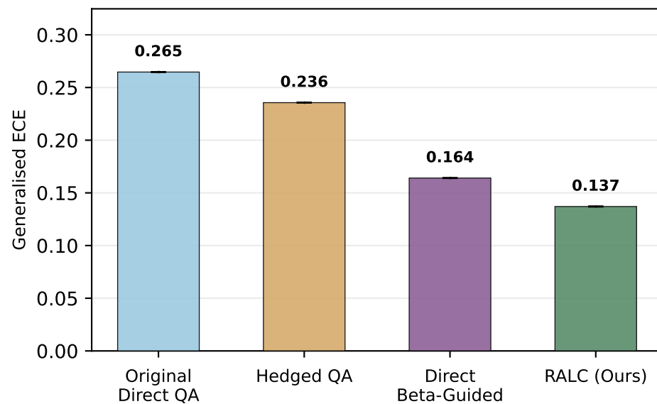
Mean Generalised ECE (Lower the Better)
