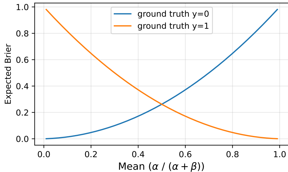
Expected Brier Fixed \alpha + \beta = 20
