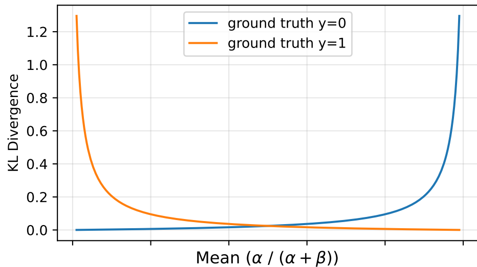
KL Divergence Fixed \alpha + \beta = 20
