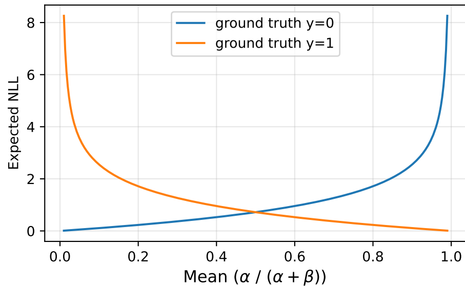
Expected NLL Fixed \alpha + \beta = 20
