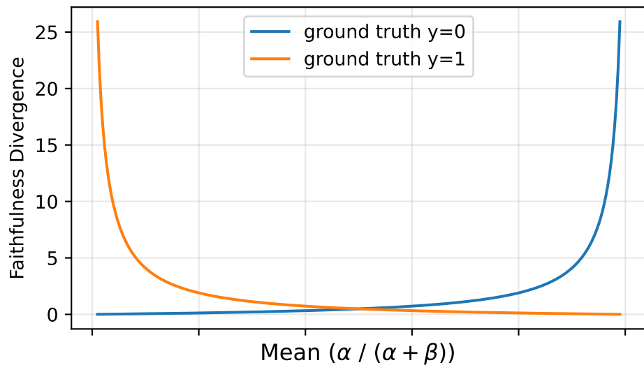
Faithfulness Divergence Fixed \alpha + \beta = 20
