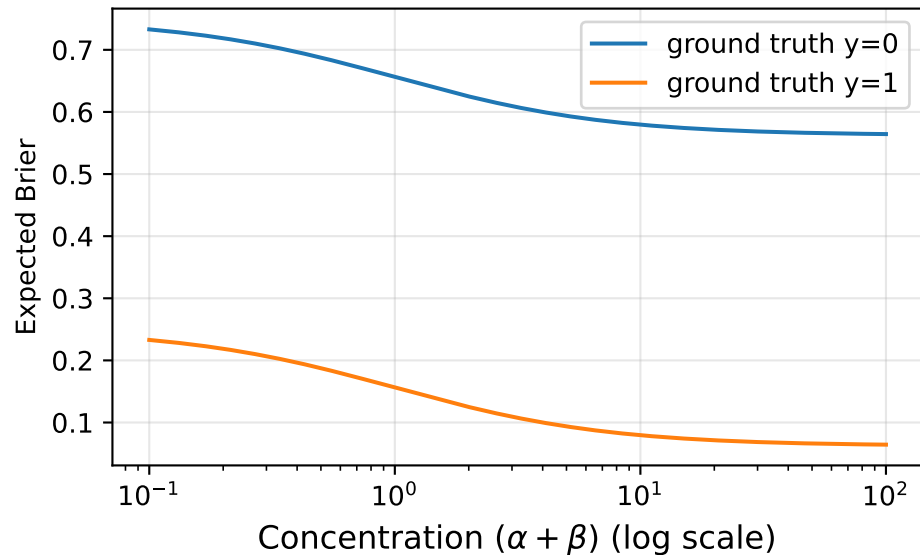
Expected Brier Fixed \mu=0.75
