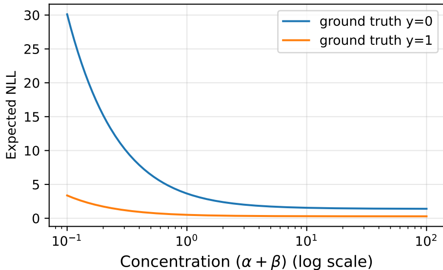
Expected NLL Fixed \mu=0.75
