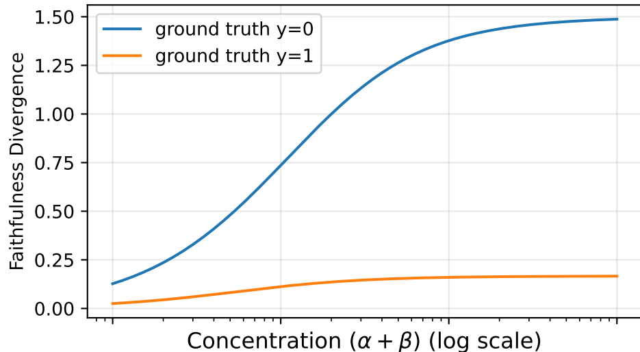
Faithfulness Divergence Fixed \mu=0.75
