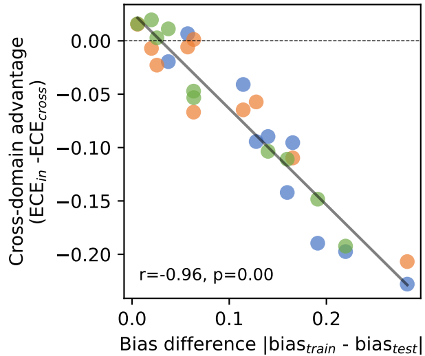
Semantic Uncertainty
