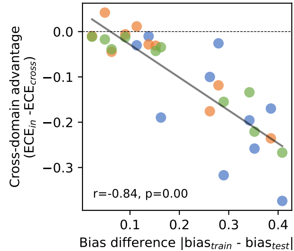
Linguistic Confidence
