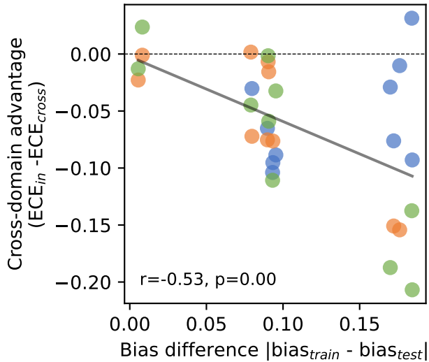
Token Probability
