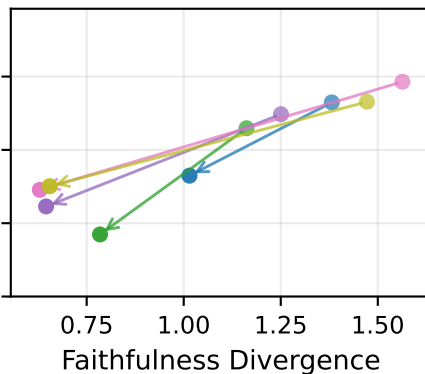
Model
