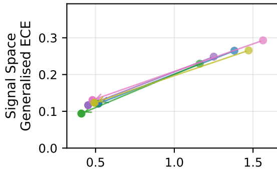
Linguistic Confidence
