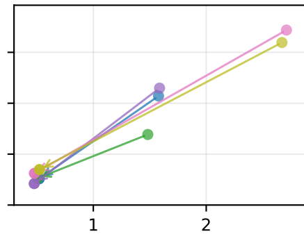
Semantic Uncertainty
