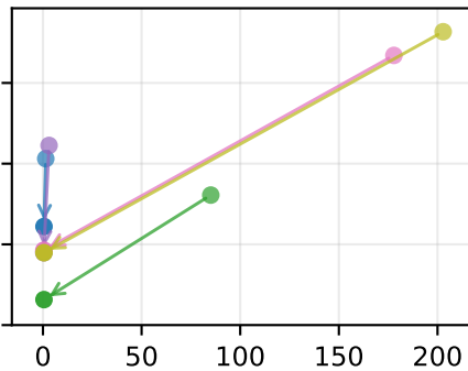
Token Probability
