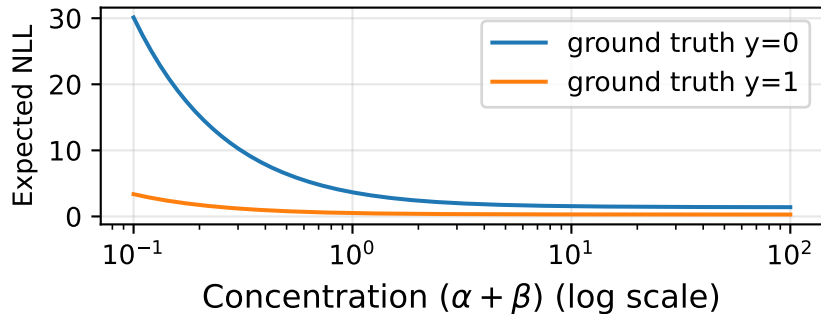
Expected NLL Fixed \mu=0.75
