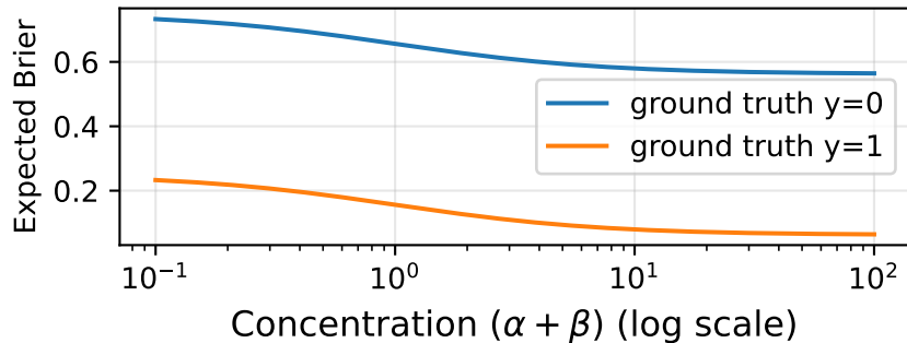
Expected Brier Fixed \mu=0.75
