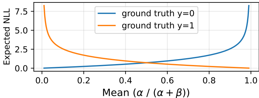
Expected NLL Fixed \alpha + \beta = 20
