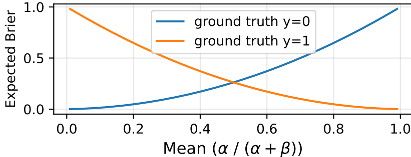
Expected Brier Fixed \alpha + \beta = 20
