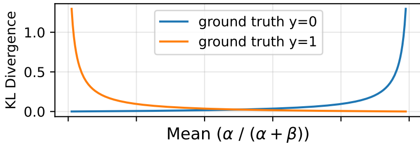
KL Divergence Fixed \alpha + \beta = 20
