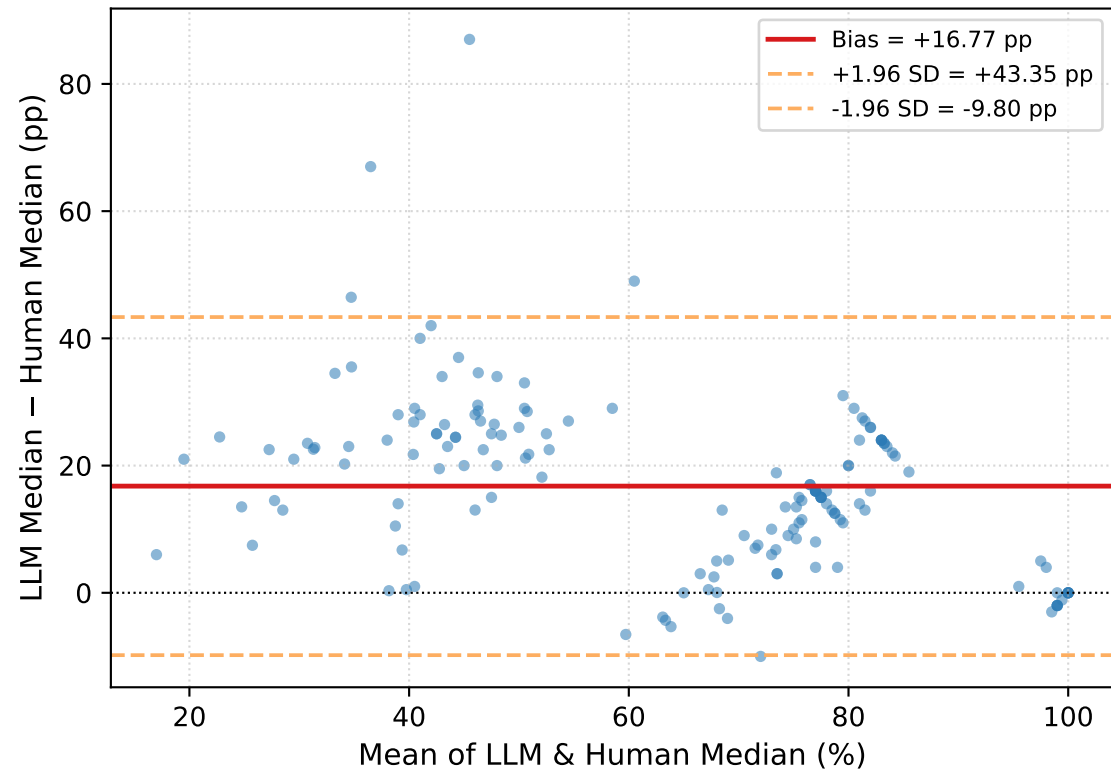
Bland-Altman Plot
