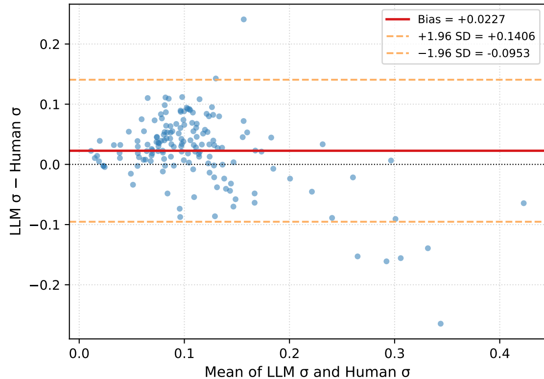
Bland-Altman: per-expression standard deviation
