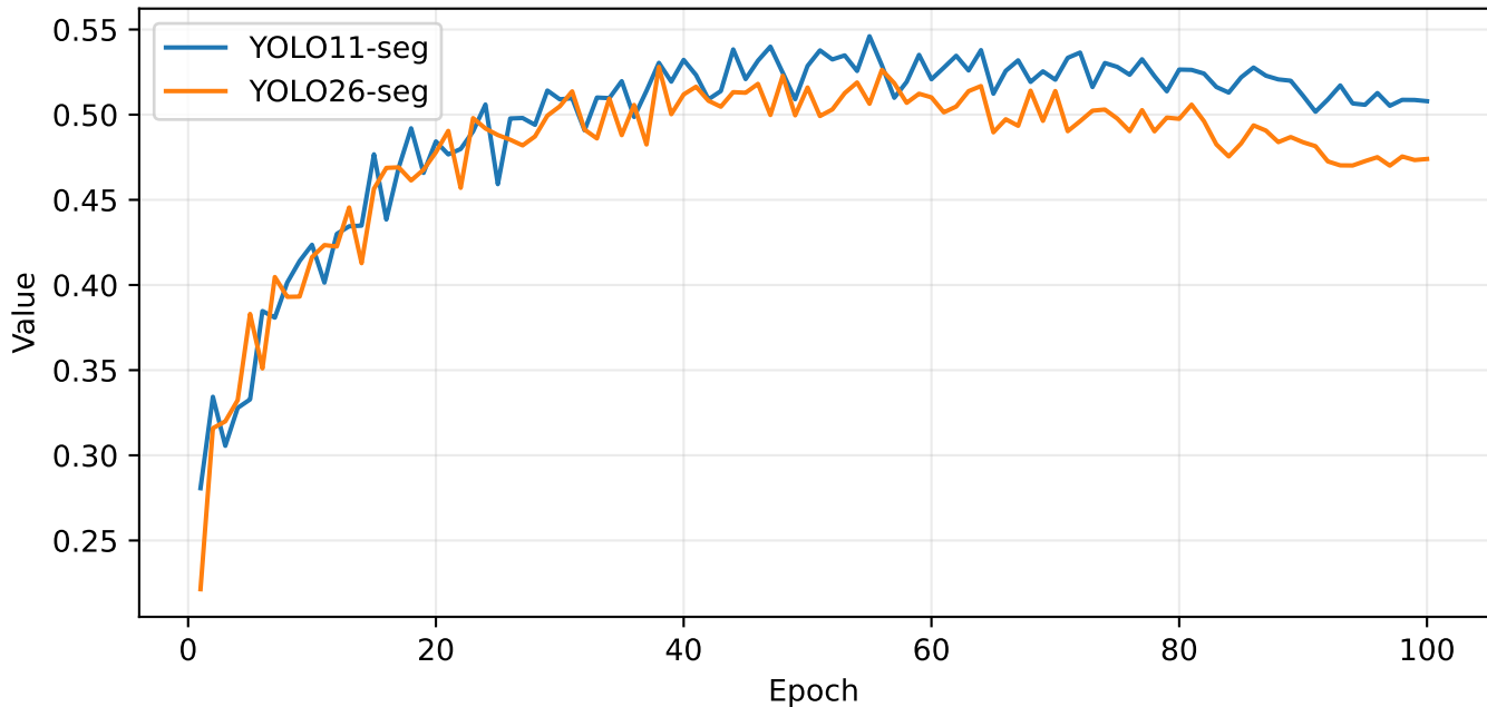
mAP50-95 (Masks)
