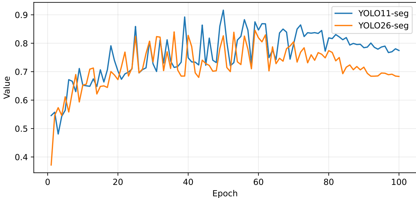
Recall (Masks)
