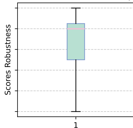
Performance Consistency
