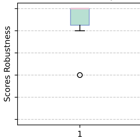
Error Recovery
