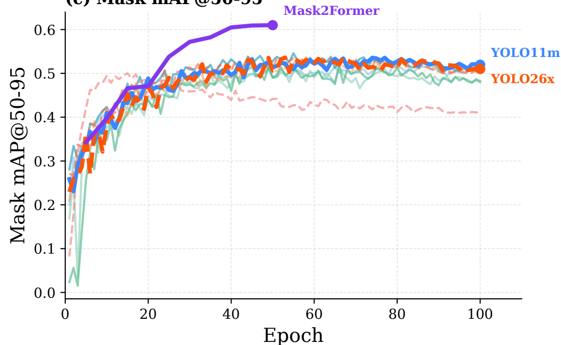
(c) Mask mAP@50-95
