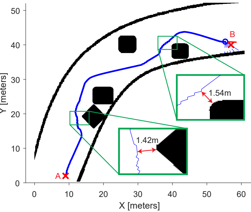
Robot Visualization
