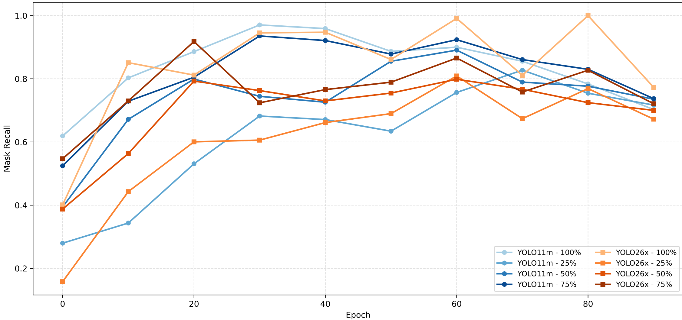
Mask Recall vs Epoch by Visibility
