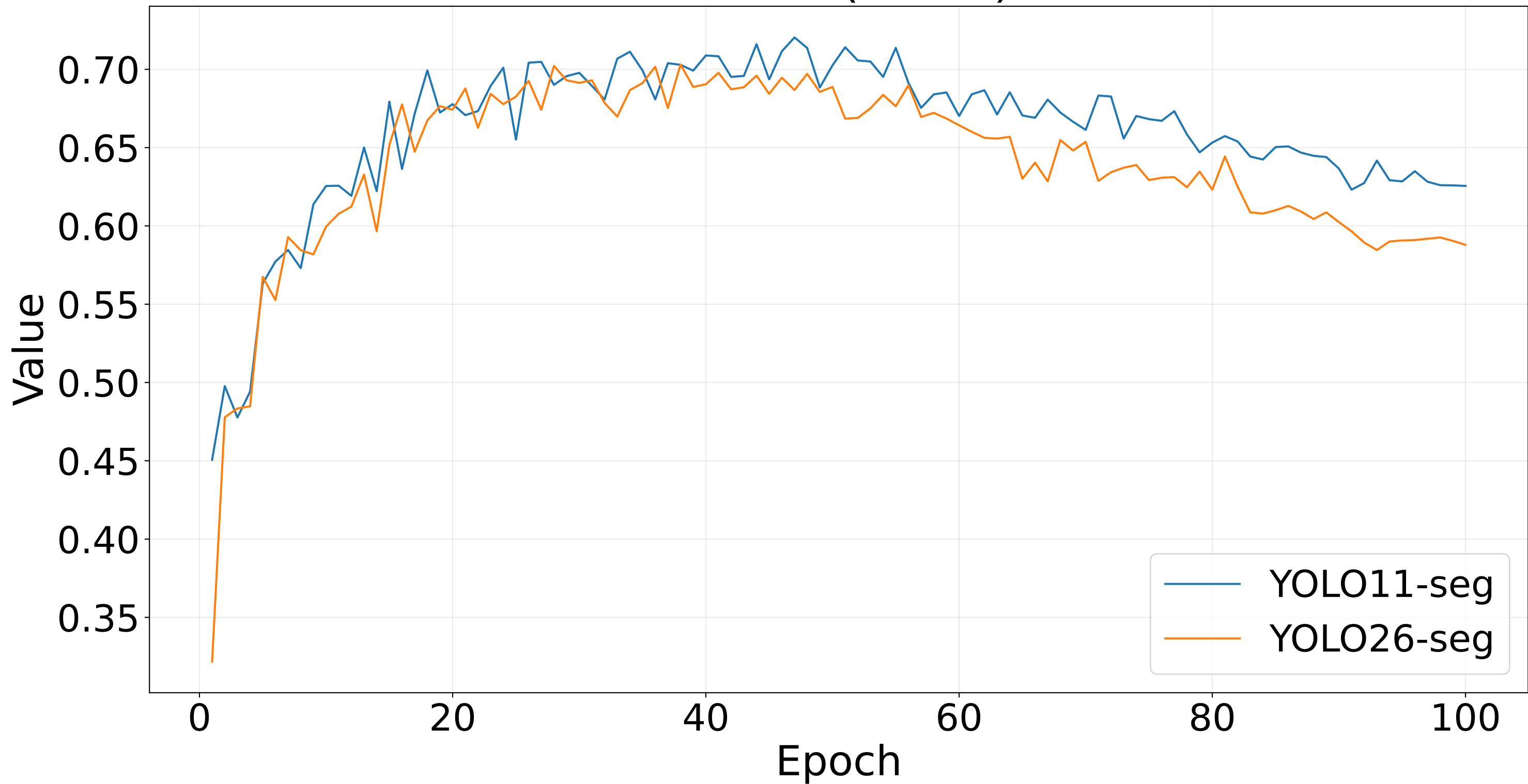
mAP50 (Boxes)
