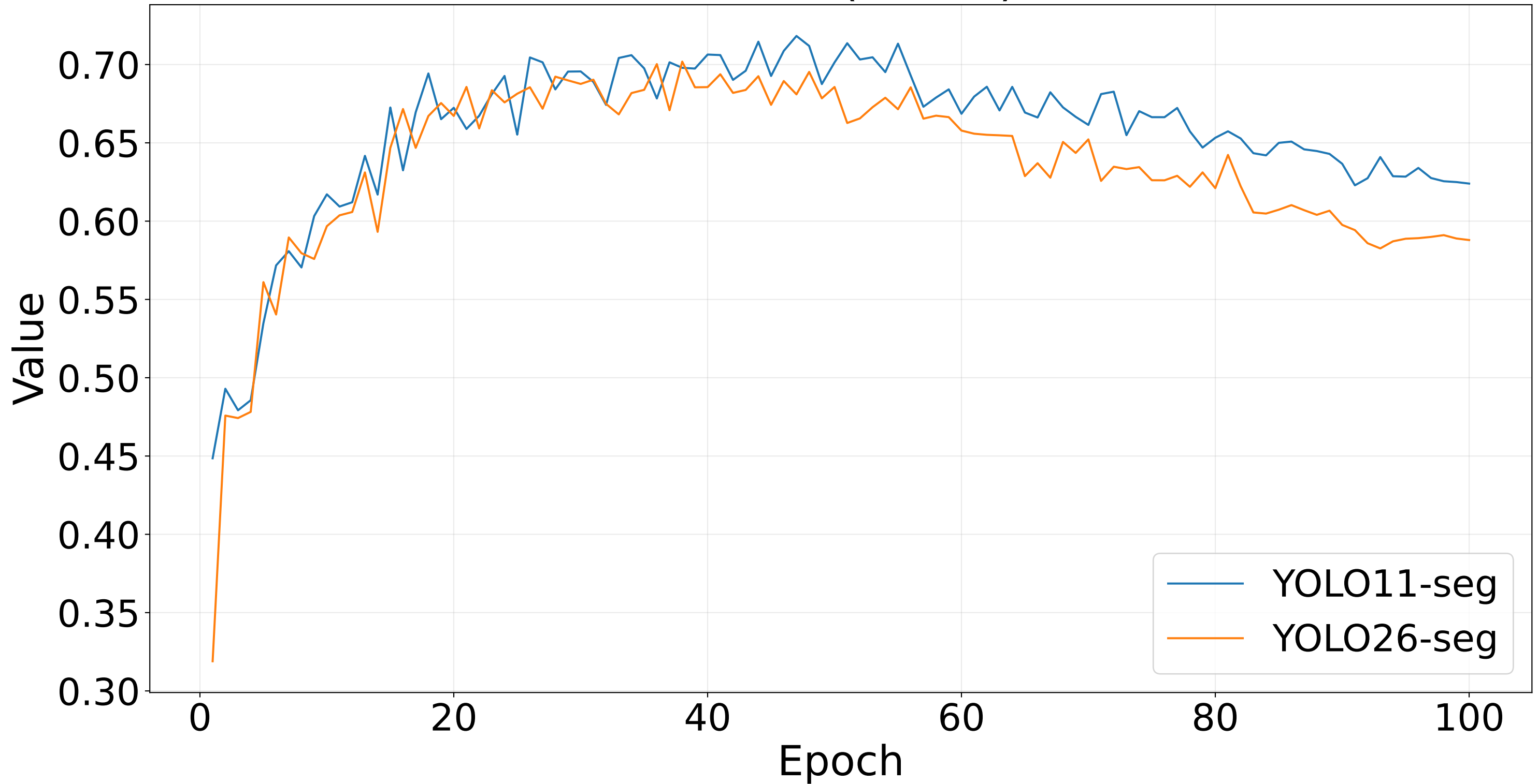
mAP50 (Masks)
