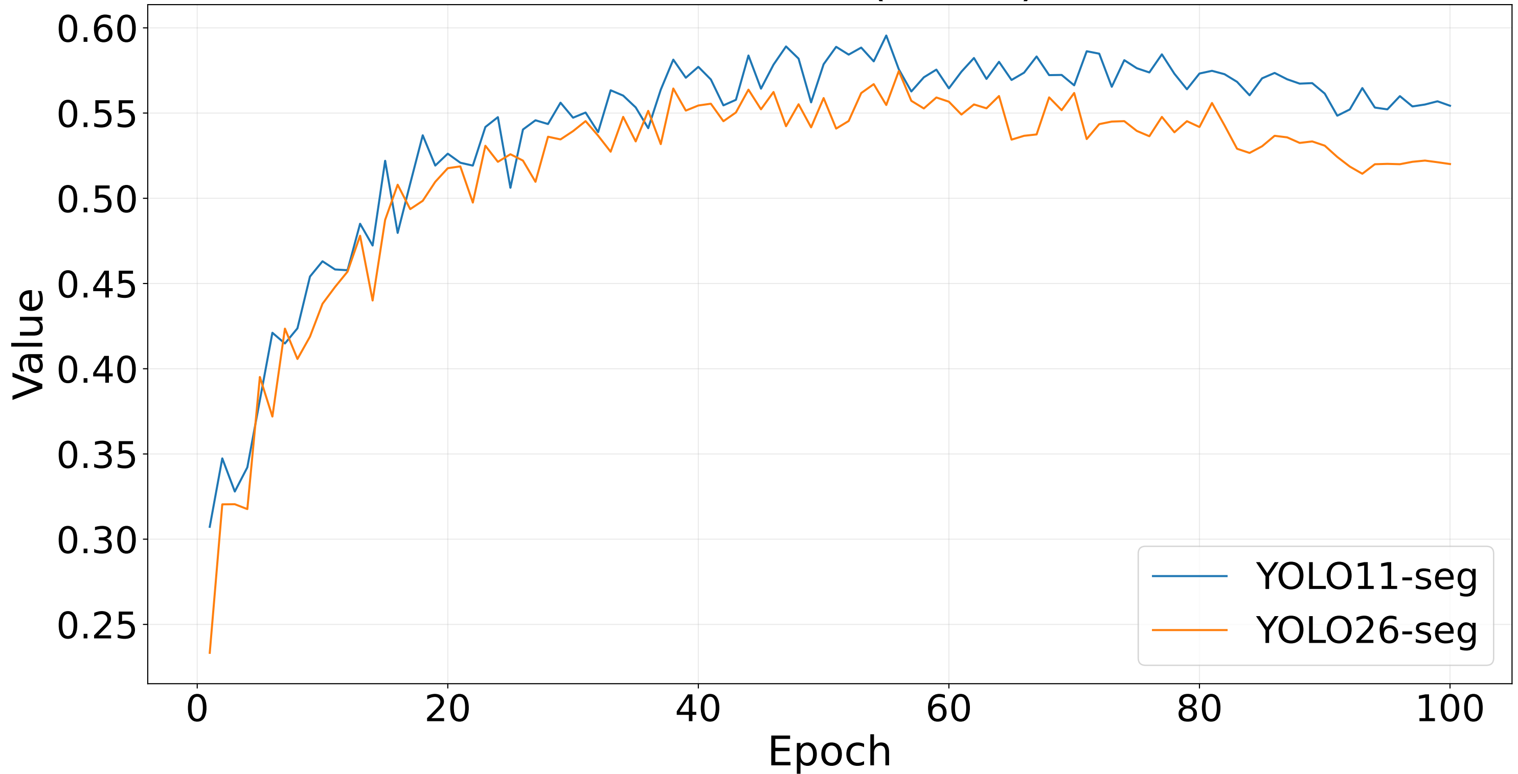
mAP50-95 (Boxes)
