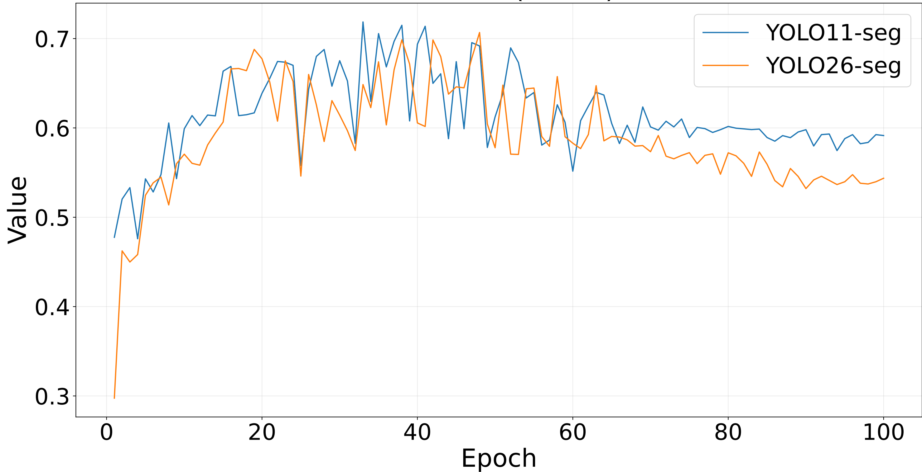
Precision (Boxes)
