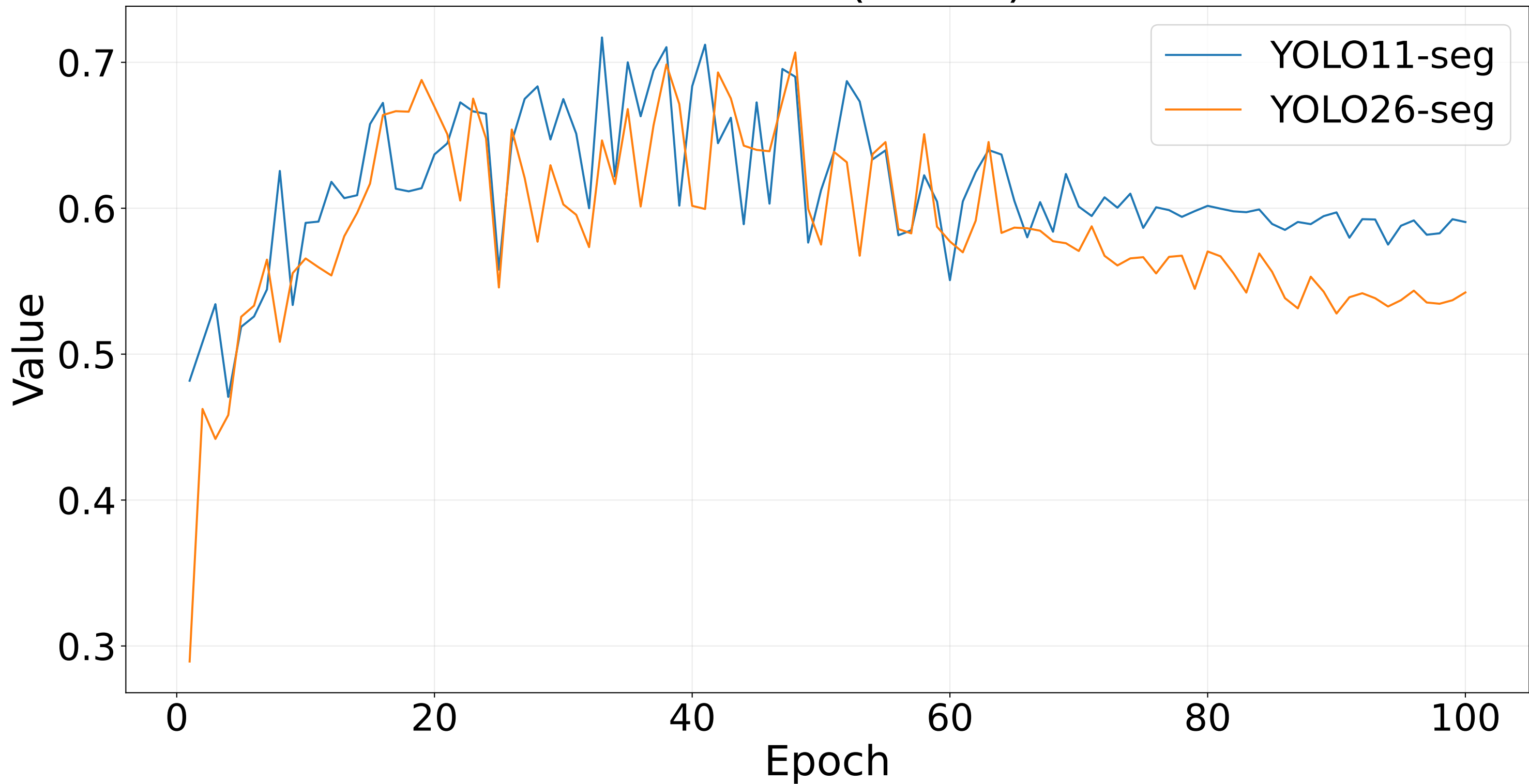
Precision (Masks)
