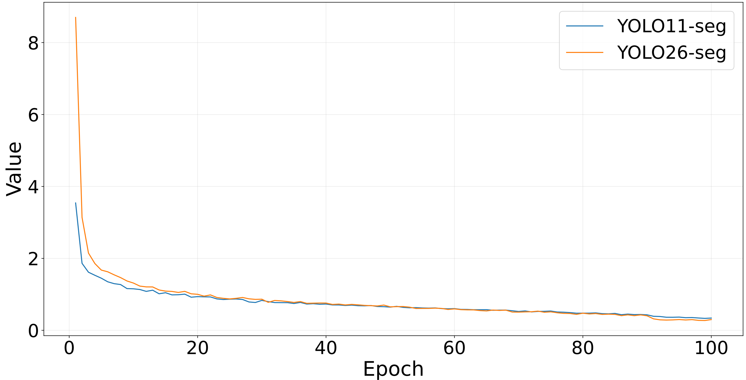
Train Cls Loss
