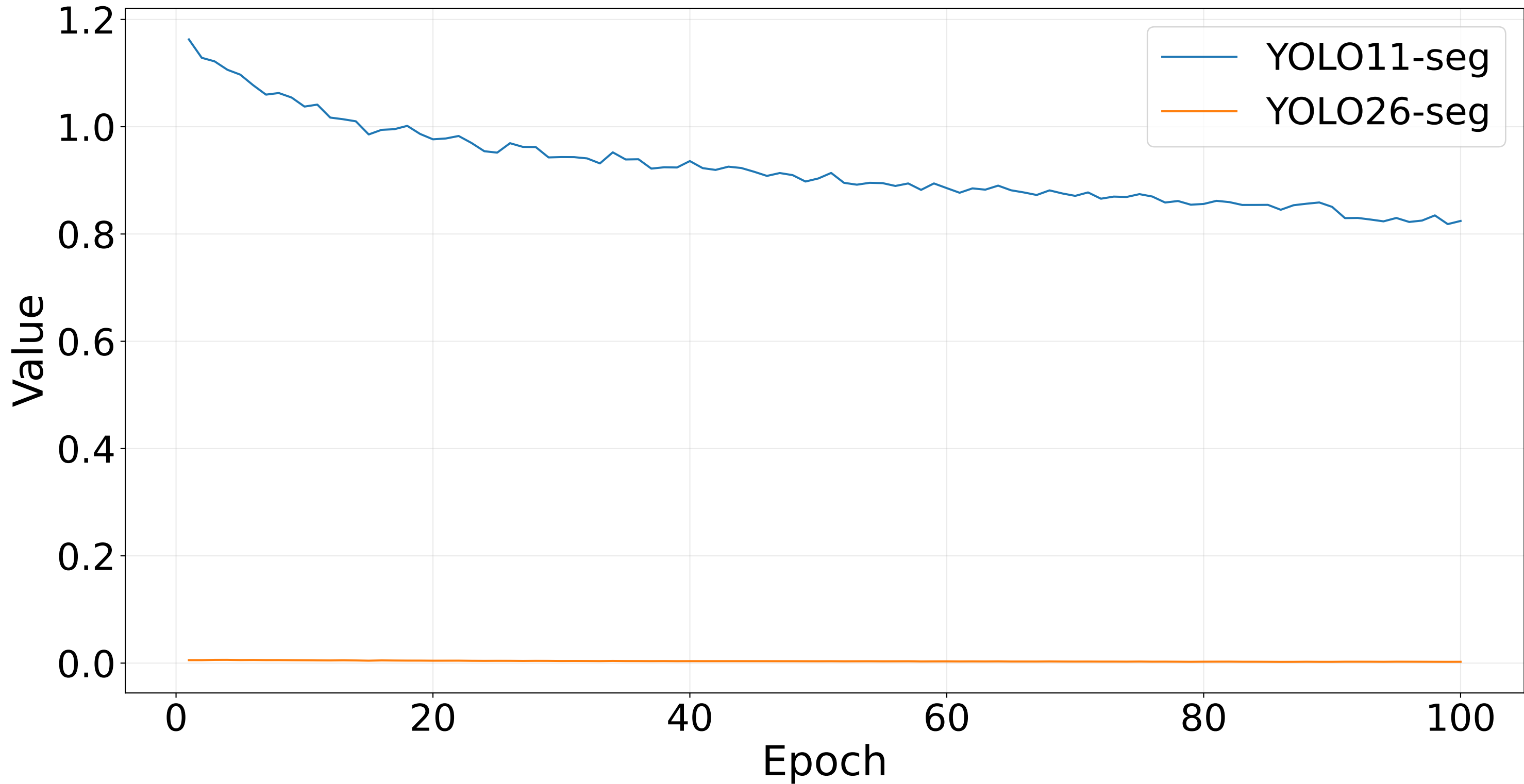
Train DFL Loss
