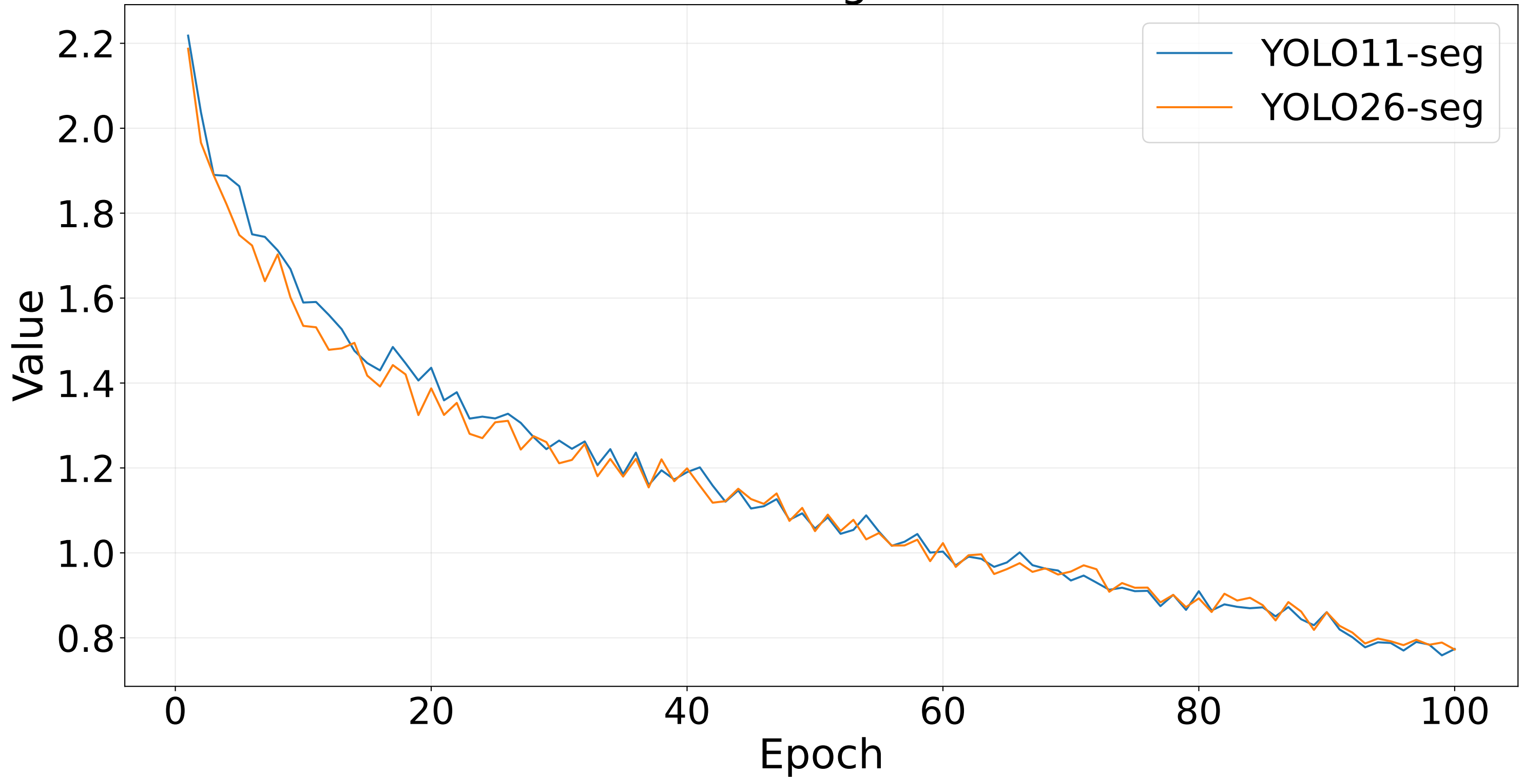
Train Seg Loss
