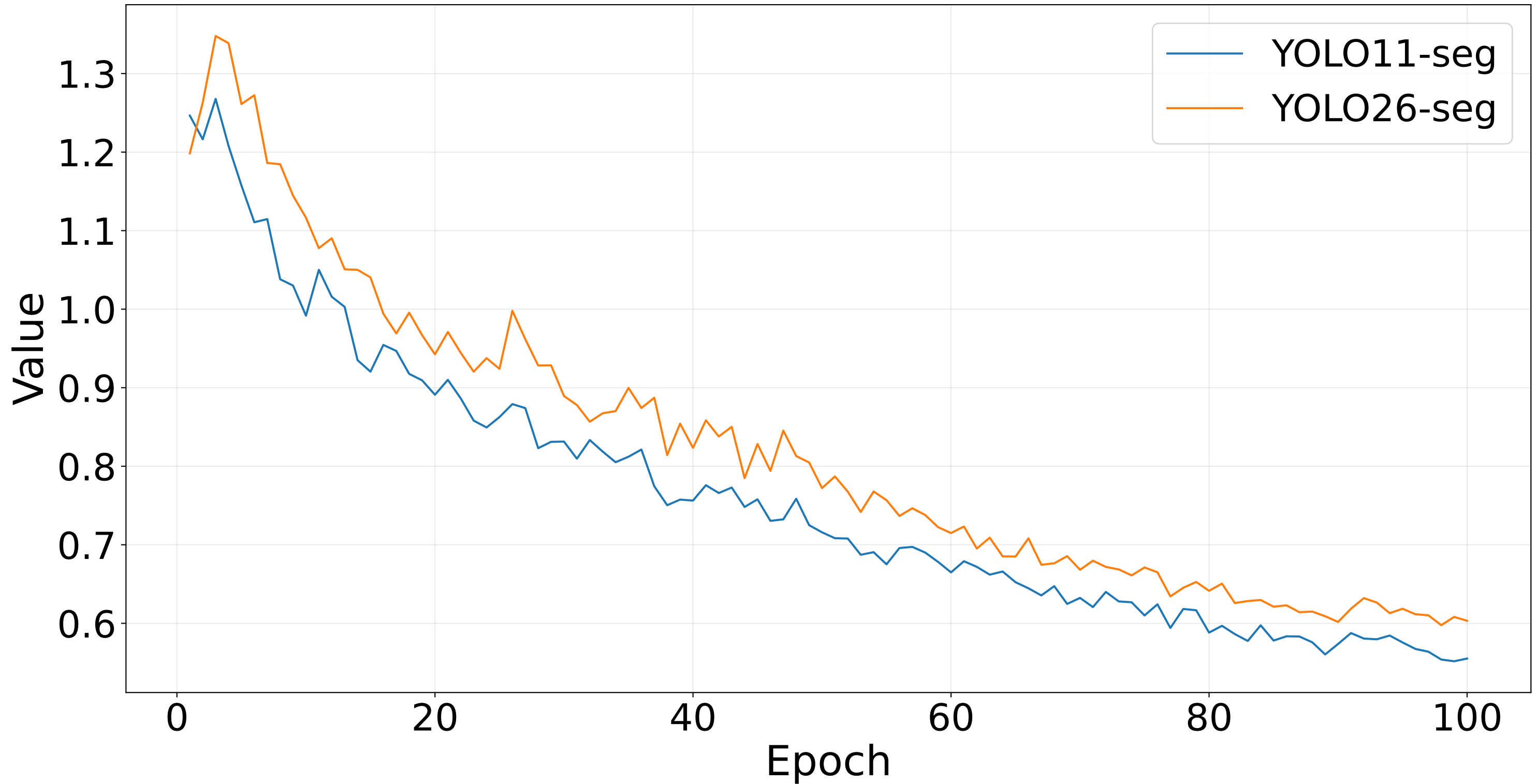
Val Box Loss
