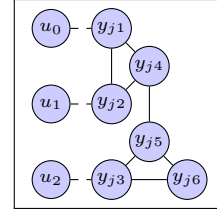
FIGURE 3 – Graphe G_0
