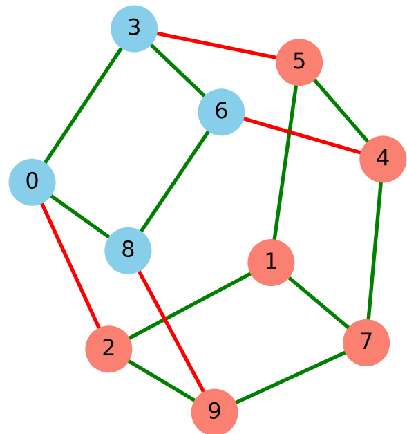
Cycle-based partition
