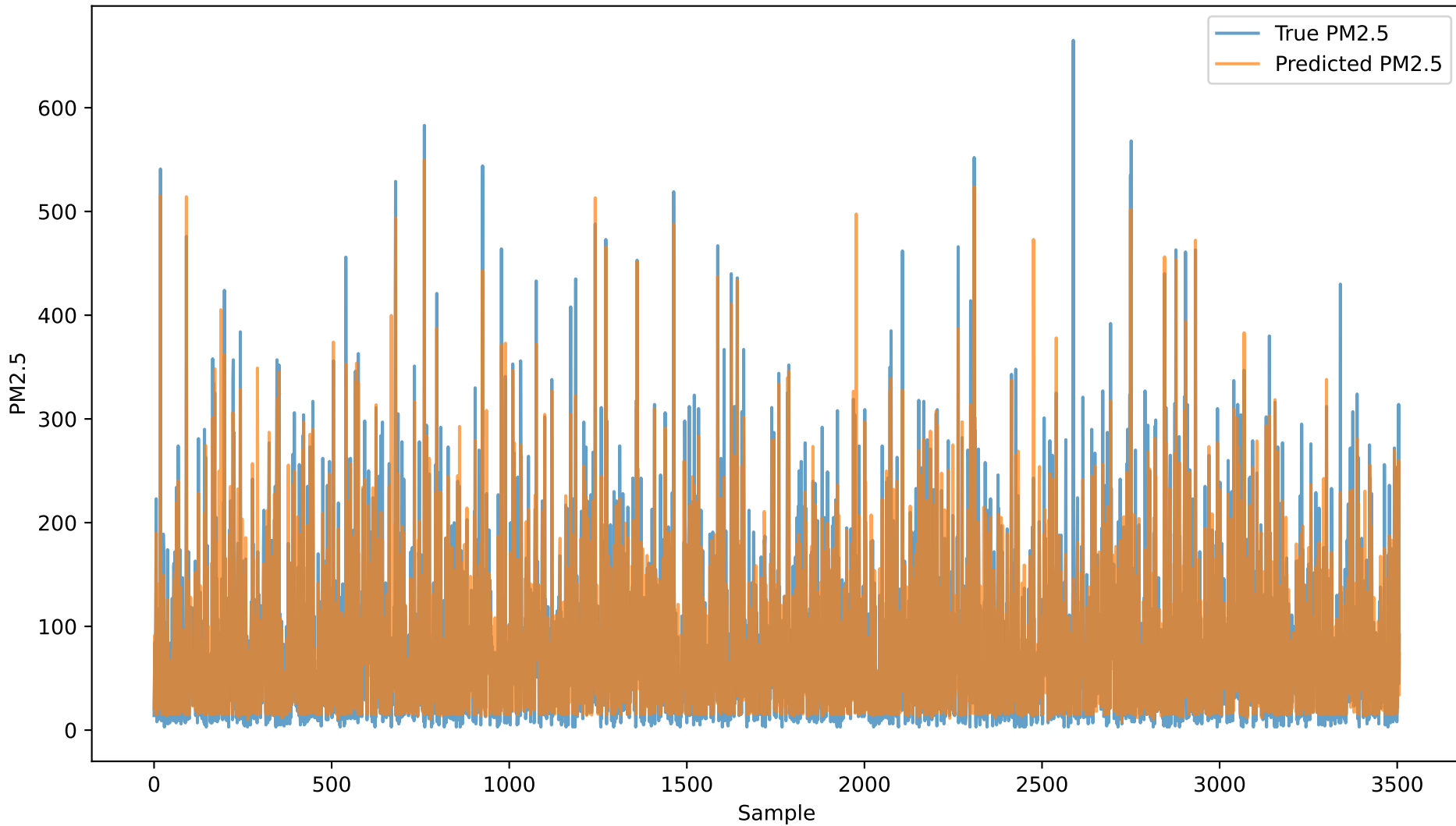
True vs Predicted PM2.5 on Test Set
