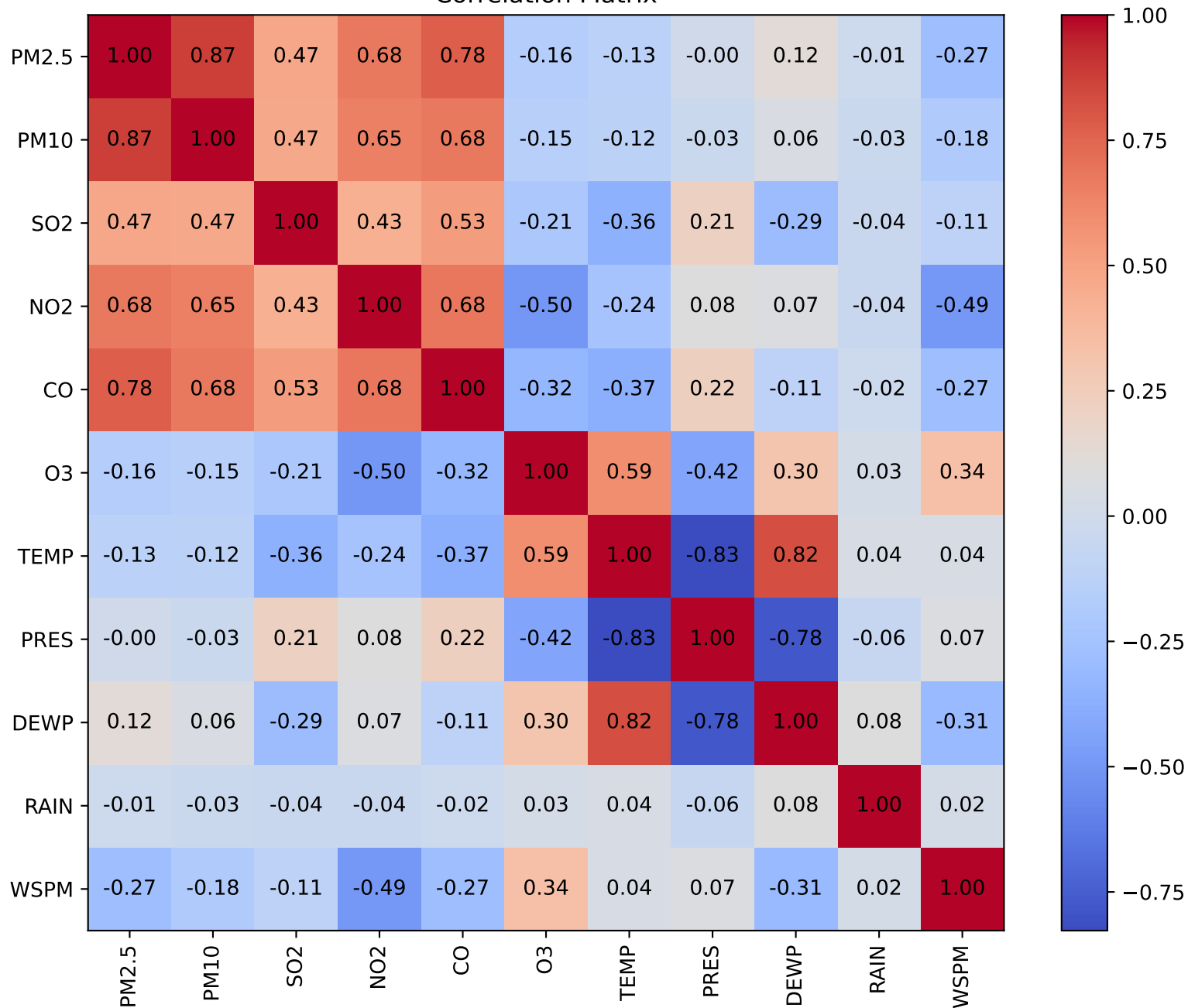
Correlation Matrix
