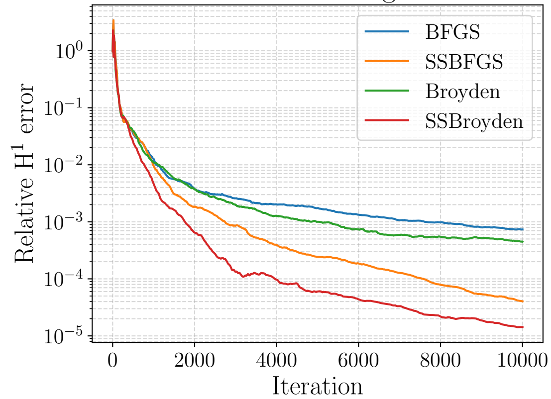
H^1 Error Convergence
