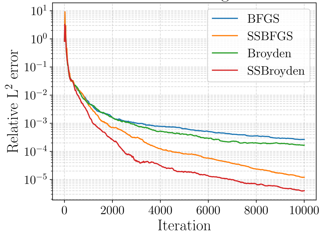
L^2 Error Convergence
