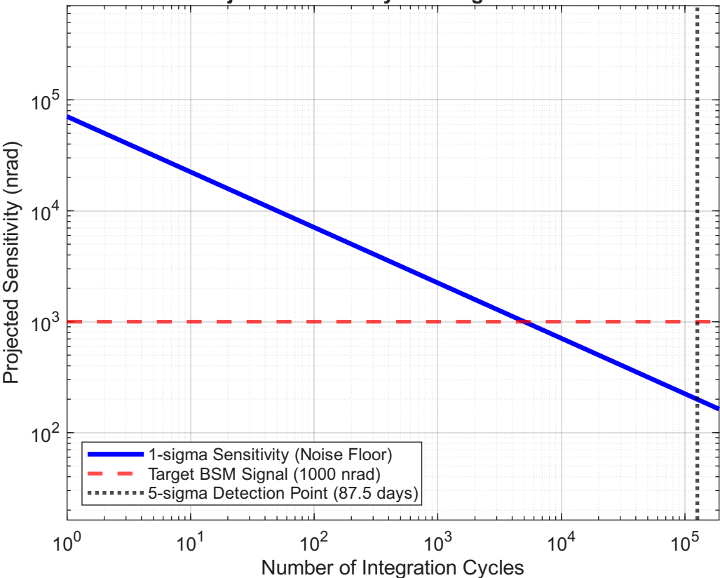
Projected Sensitivity vs. Integration Time
