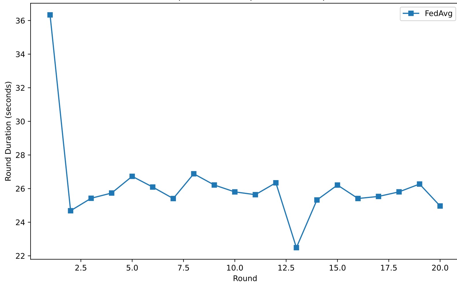
Time per Round Comparison - oxfordpet
