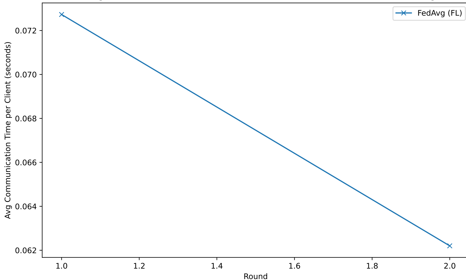
Average Client Communication Time - stl10 (Model: resnet, Federated Learning)
