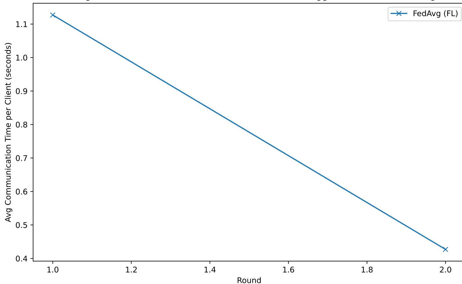
Average Client Communication Time - cifar10 (Model: vgg16, Federated Learning)
