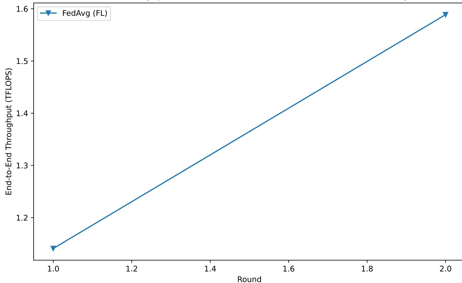
Round Throughput TFLOPS - stl10 (Model: resnet, Federated Learning)
