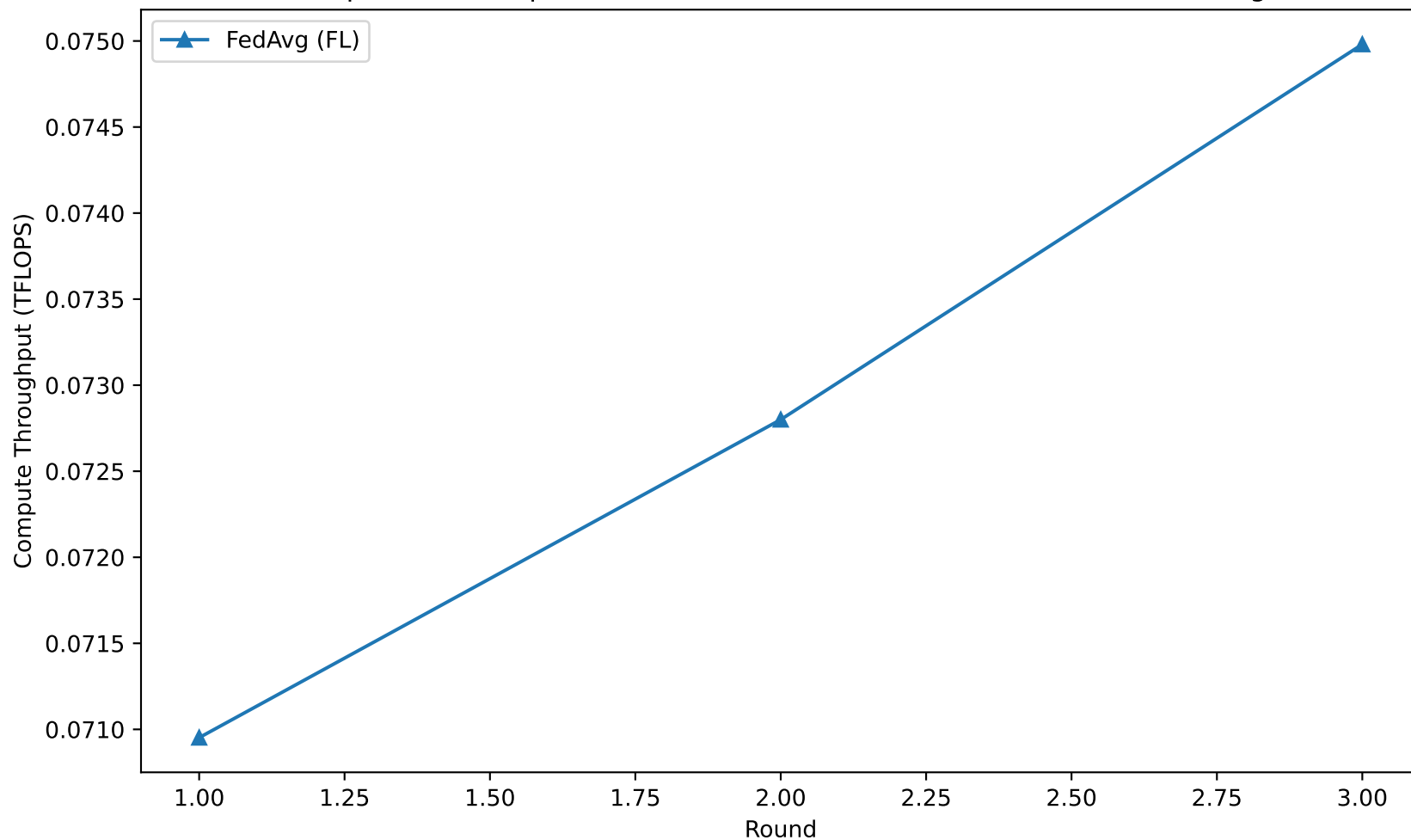
Compute TFLOPS per Round - mnist (Model: resnet, Federated Learning)
