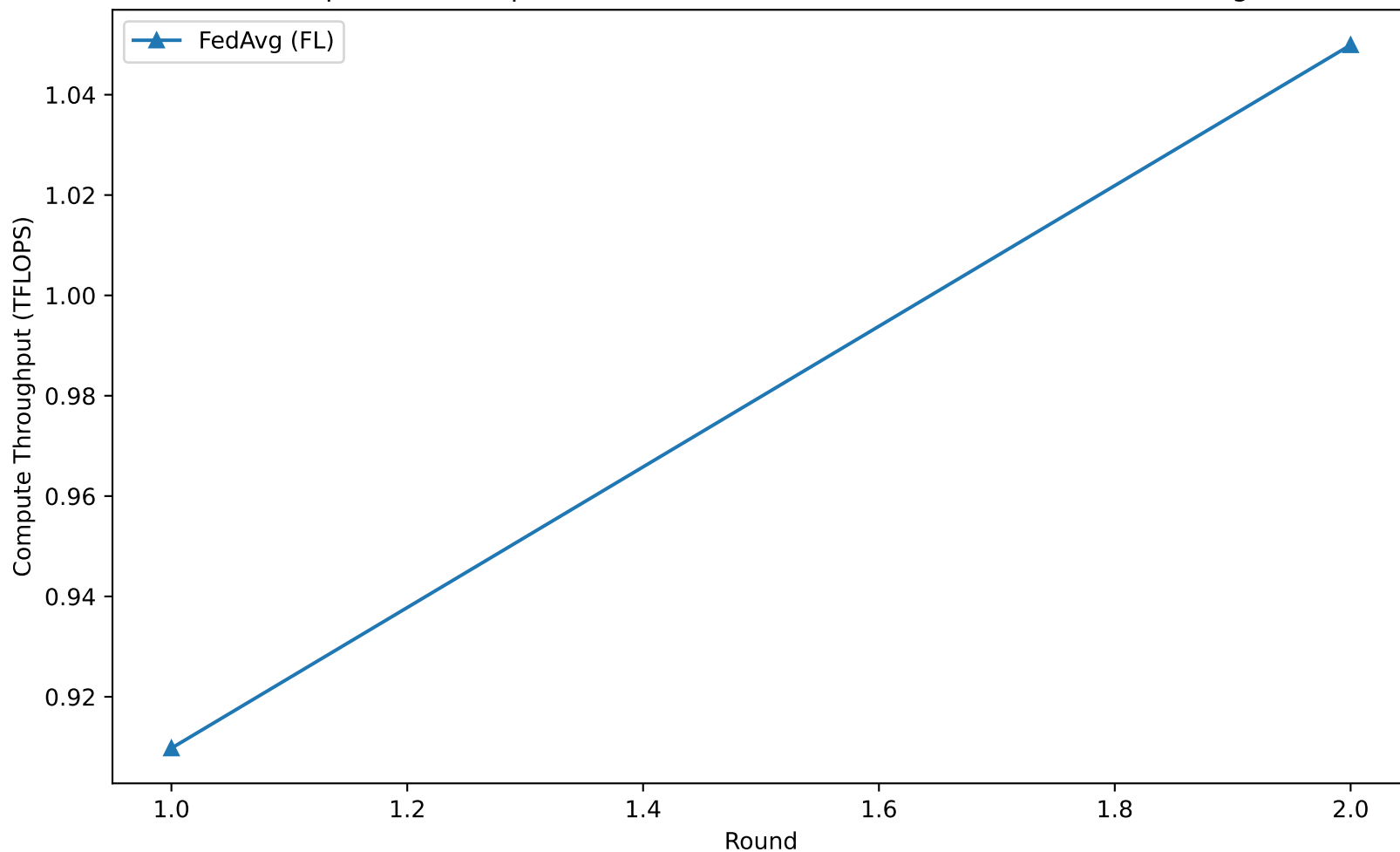
Compute TFLOPS per Round - stl10 (Model: resnet, Federated Learning)
