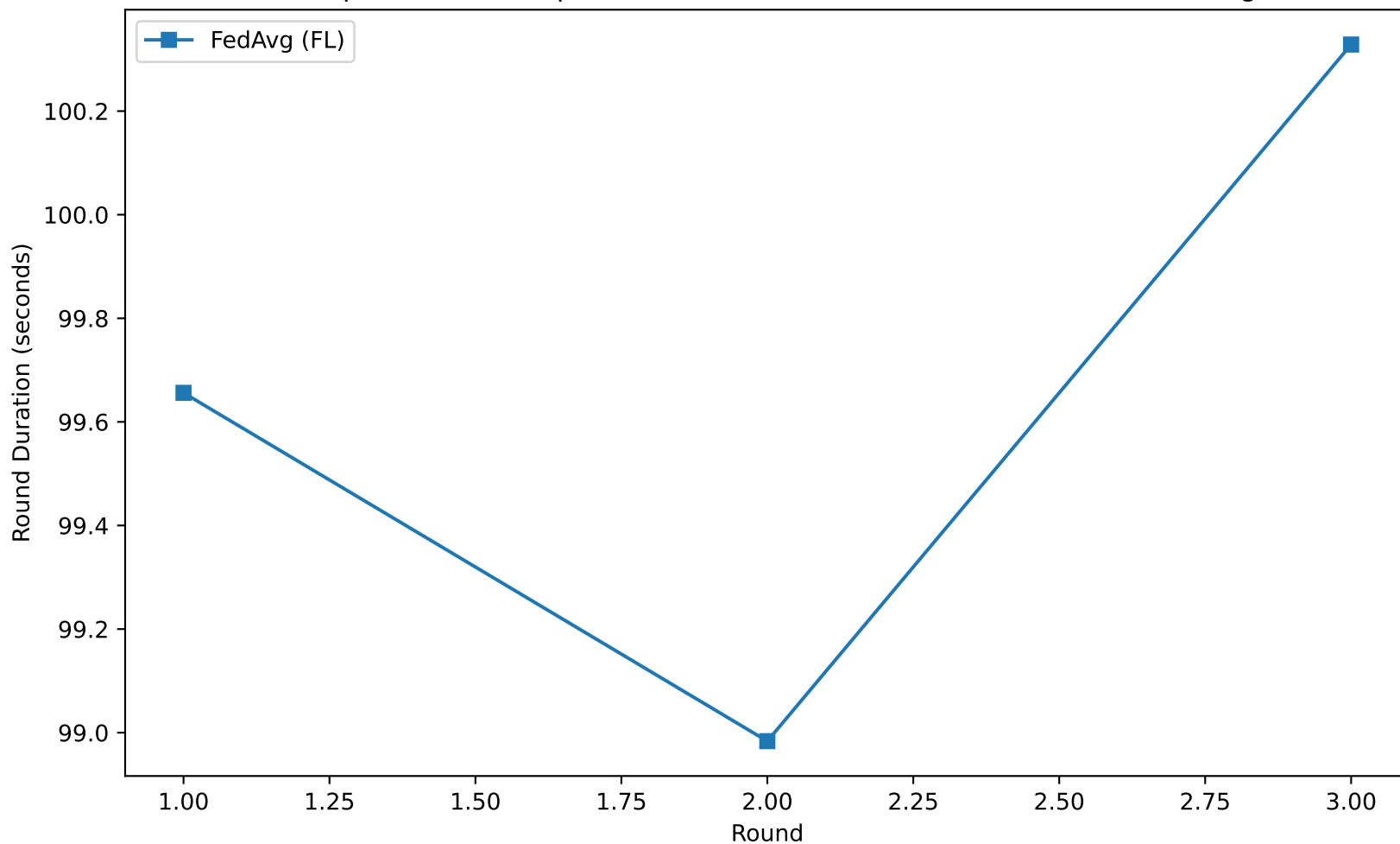
Time per Round Comparison - mnist (Model: resnet, Federated Learning)
