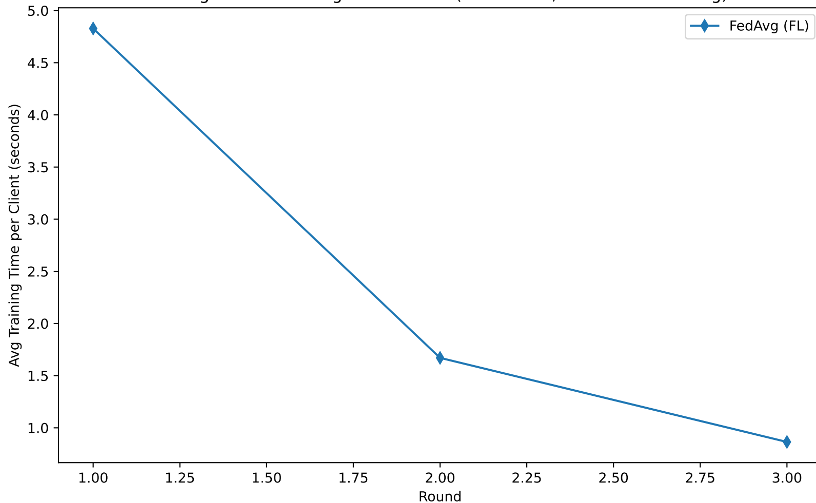
Average Client Training Time - mnist (Model: cnn, Federated Learning)
