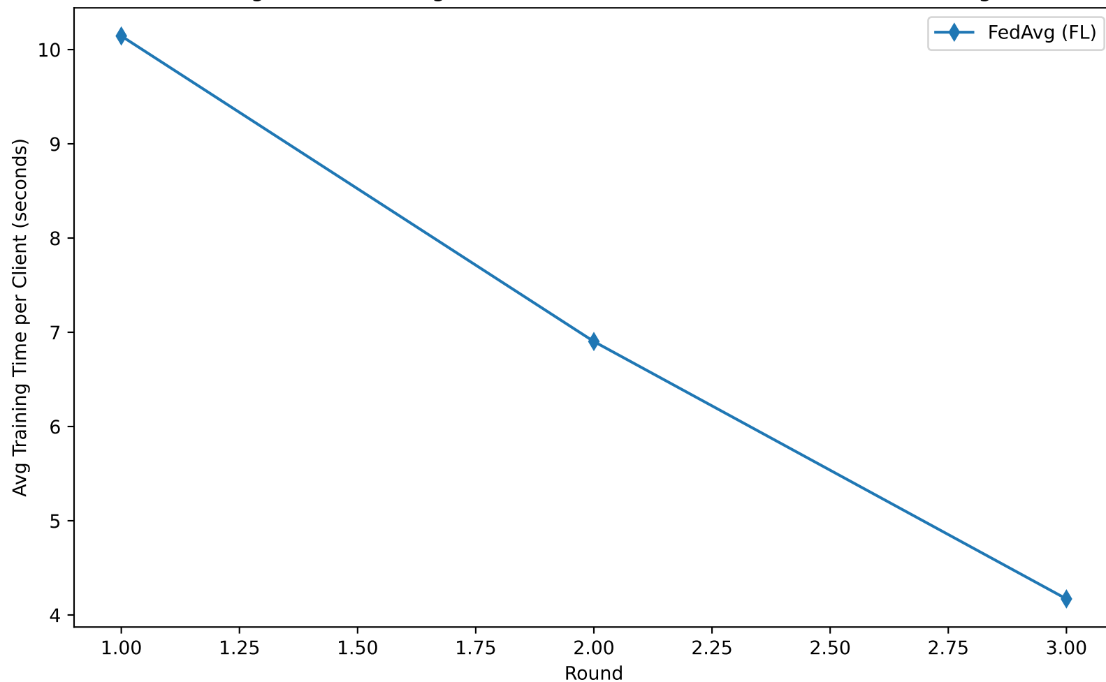
Average Client Training Time - mnist (Model: resnet, Federated Learning)
