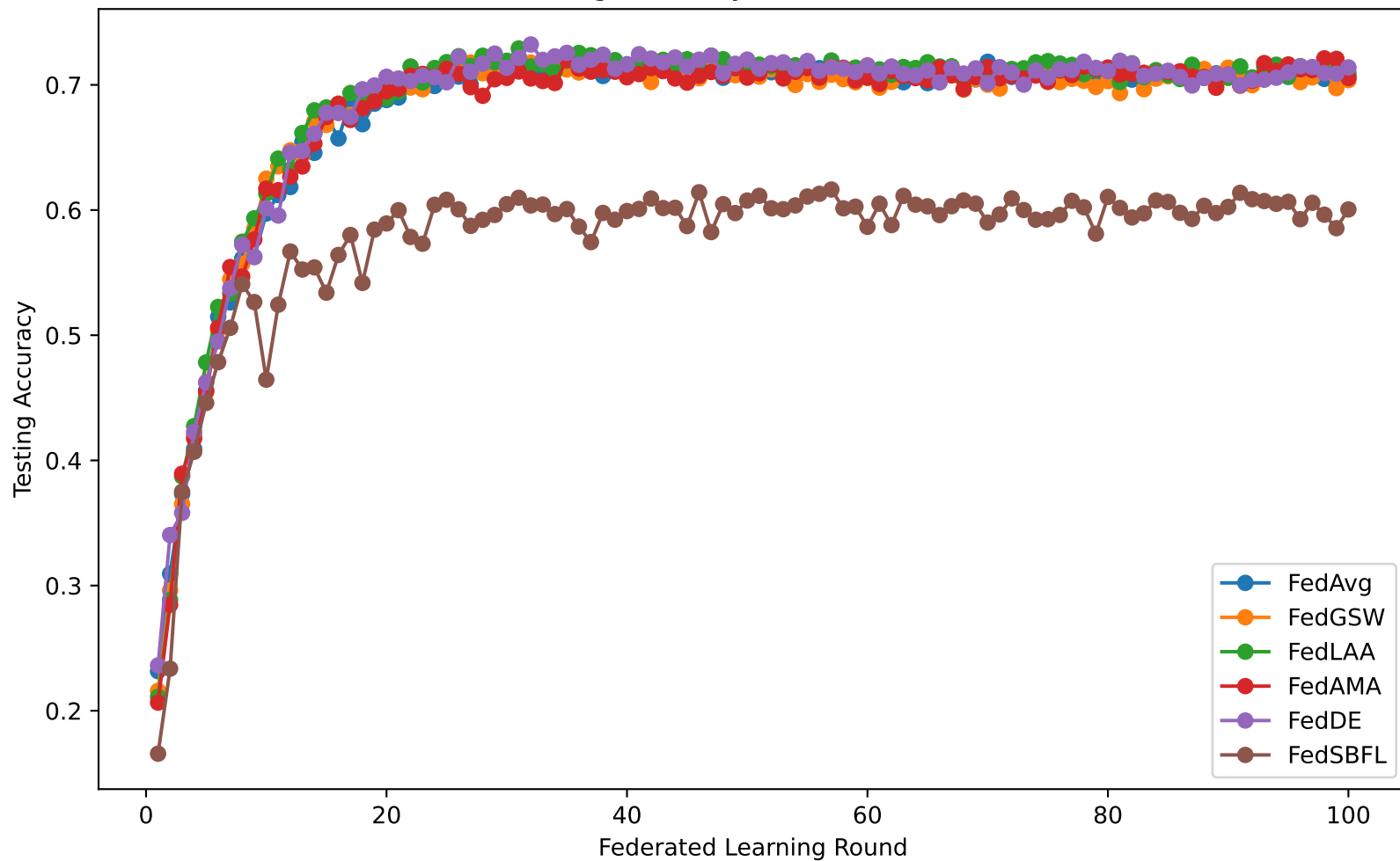
Testing Accuracy - cnn and cifar10
